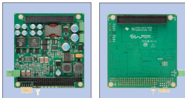
Front and Back Picture of PPM-DC-ATX-P
